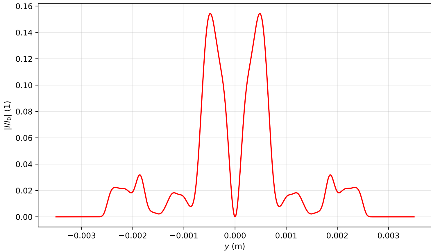
Intensity profile I(x = 0, y, z = 3.821)/I_0 , P_{in}=8.0P_{cr} , artificial time
